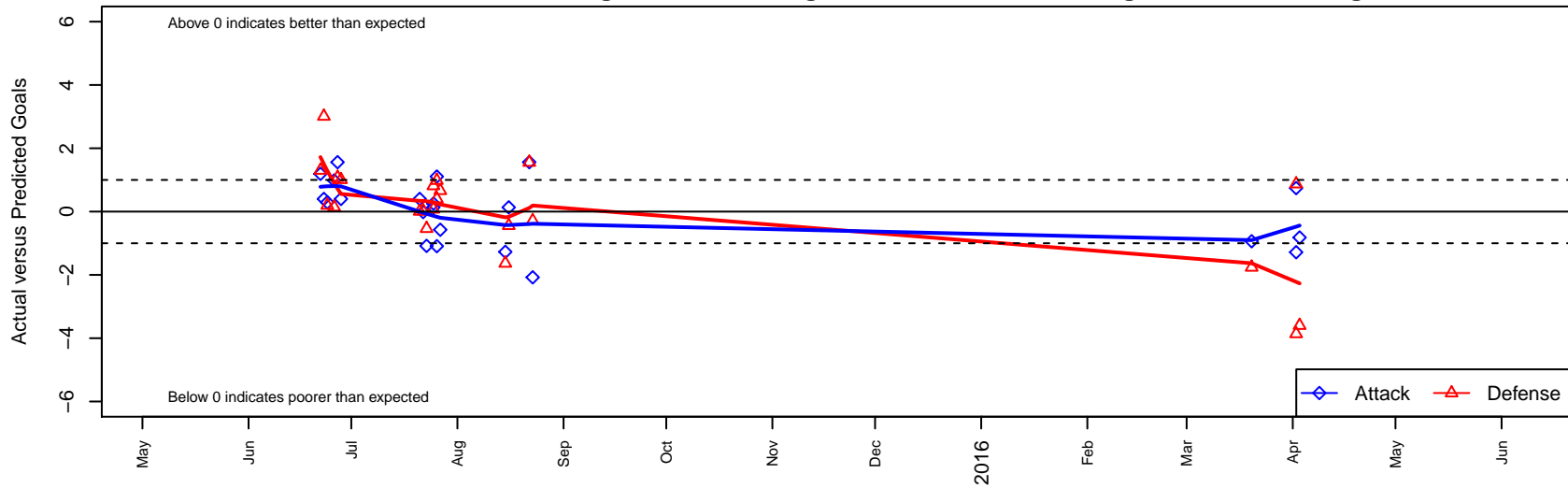
Albion SC White B98 Dots are actual minus expected GF (blue circles) and GA (red triangles). Blue line is smoothed change in attack strength. Red is smoothed change in defense strength.
